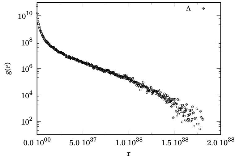
FIG. 1. The RDF for case A of Table I. The radial distance r is in Planck units 1.61623 \times 10^{-33} cm. A logarithmic scale is used on the y -axis.
