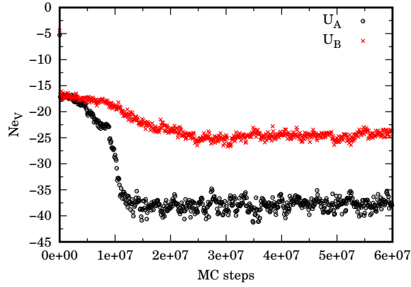
FIG. 9. We show the evolution of the potential energy Ne_V during the simulation of case E\mathcal{A} ( U_{\mathcal{A}} ) and E\mathcal{B} ( U_{\mathcal{B}} ). The energy is in units of a Hartree. For case E\mathcal{A} we see an abrupt ‘transition’ at about 10^7 MC steps when the blob shown in Fig. 8 is formed.
