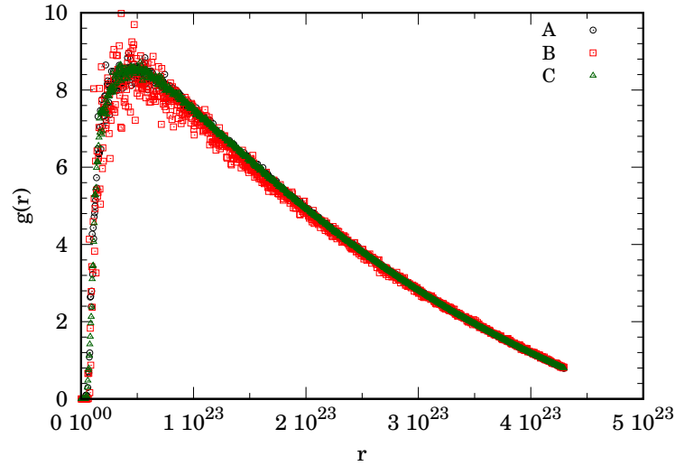
FIG. 1. The RDF for cases A,B,C of Table I without permutations. The radial distance r is in Planck units 1.61623 \times 10^{-33} cm. The radial length of the patch is \delta = 4.3 \times 10^{23} .
