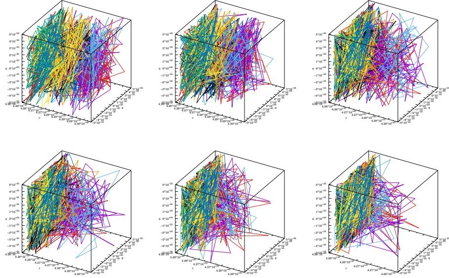
FIG. 1. Evolution of the simulation of case A of Table I during the run. Reading from up to bottom, left to right we show snapshots at 3 \times 10^4 , 5 \times 10^4 , 8 \times 10^4 , 9 \times 10^4 , 11 \times 10^4 , 13 \times 10^4 , MC steps. The paths of the 50 electrons are painted with different colors.
