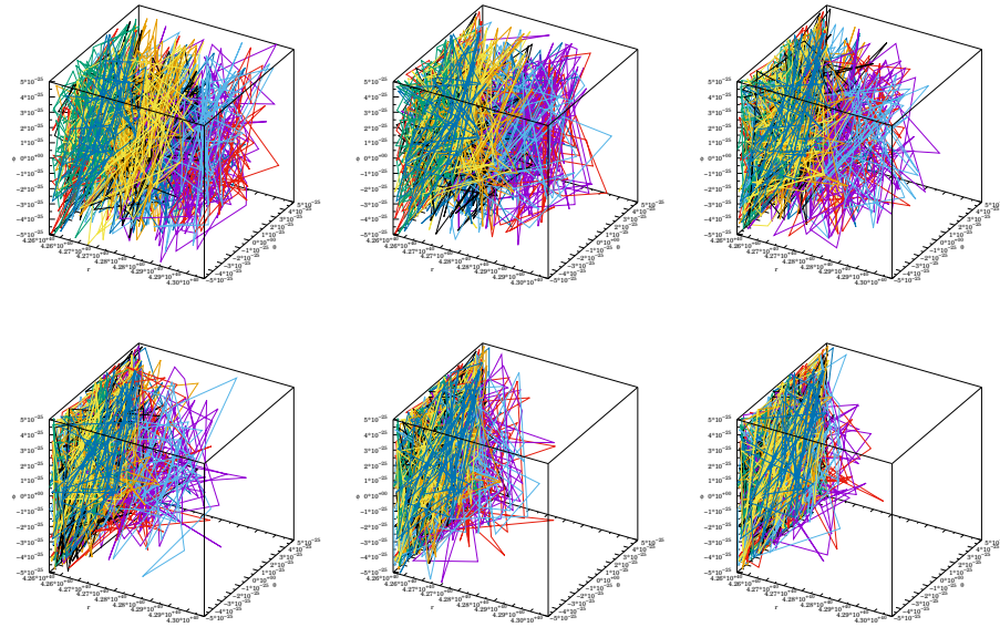
FIG. 1. Evolution of the simulation of case A of Table I during the run. Reading from up to bottom, left to right we show snapshots at 300, 500, 700, 900, 1100, 1300 MC steps. The paths of the 30 electrons are painted with different colors.
