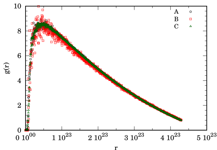
FIG. 1. The RDF for cases A,B,C of Table I without permutations. We explicitly verified that taking into account the permutations among the electrons does not change appreciably the RDF. The RDF of cases M and BH is also not appreciably different from the one of case A shown here. The radial distance r is in Planck units 1.61623 \times 10^{-33} cm. The radial length of the patch is \delta = 4.3 \times 10^{23} .
