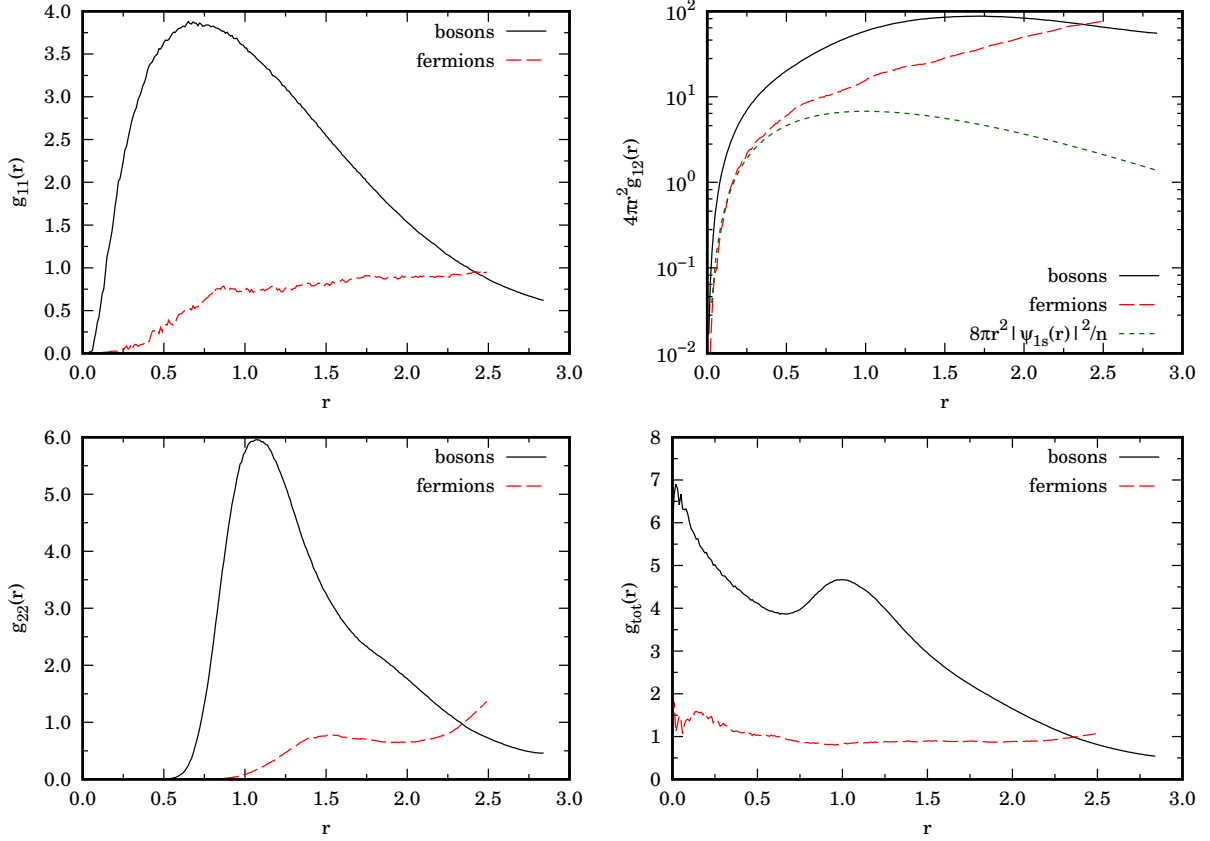
FIG. 7. We show the partial and total RDF of the H fluid for cases E \mathcal{B} and F \mathcal{B} in Table I where \tau = 0.3 . In the panel for the unlike radial distribution function we also show the ground state probability distribution of the H atom |\psi_{1s}|^2 for comparison. The distance r is in units of a Bohr radius.
