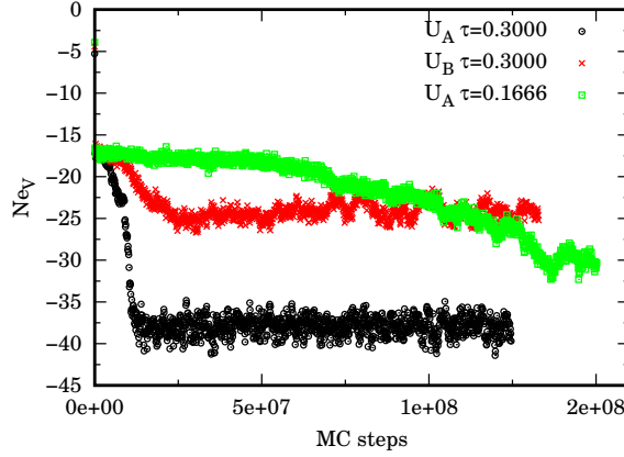
FIG. 9. We show the evolution of the potential energy NeV during the simulation of case E \mathcal{A} ( U_{\mathcal{A}} \tau = 0.3 ) and E \mathcal{B} ( U_{\mathcal{B}} \tau = 0.3 ) and for the same bosonic mixture treated with the inter-action \mathcal{A} with a smaller timestep \tau = 0.1666 for M = 200 . For case E \mathcal{A} with \tau = 0.3 we see an abrupt ‘transition’ at about 10^7 MC steps when the blob shown in Fig. 8 is formed. The energy is in units of a Hartree.
