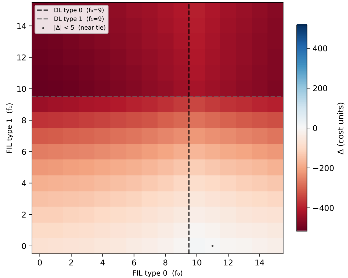
\Delta = Q(\text{serve 1}) - Q(\text{serve 0}) blue = type 0 cheaper \triangleright serve 0 | red = type 1 cheaper \triangleright serve 1
