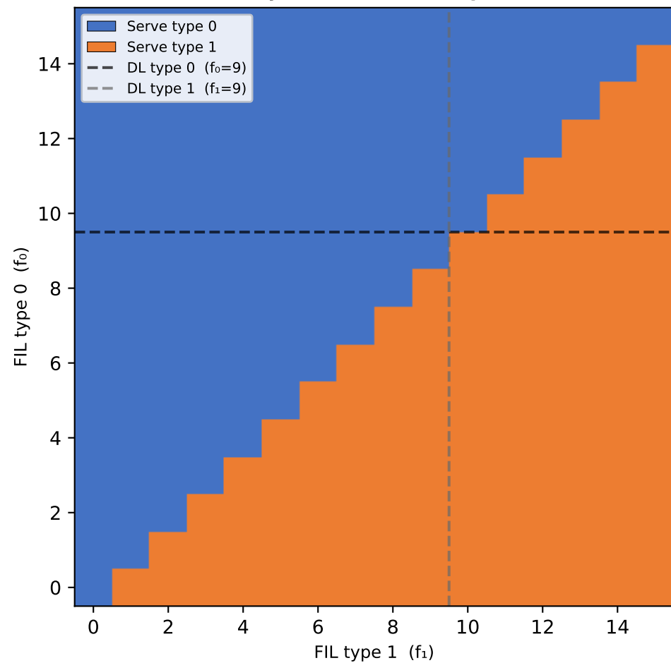
FIFO policy (always serves head-of-queue)
