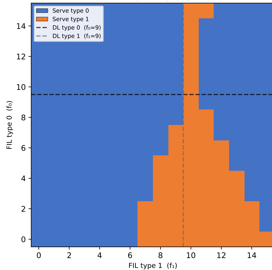
RVI optimal policy
