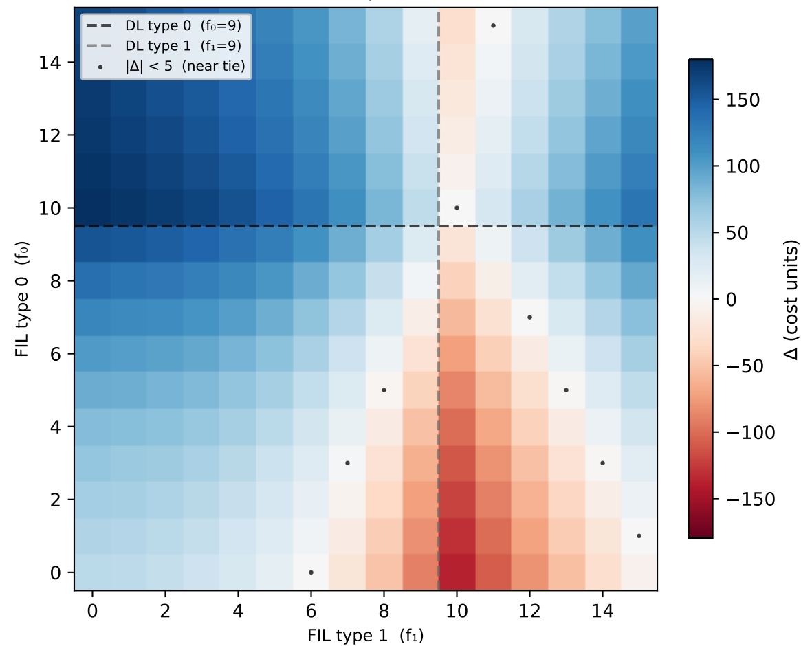
\Delta = Q(\text{serve 1}) - Q(\text{serve 0}) blue = type 0 cheaper \triangleright serve 0 | red = type 1 cheaper \triangleright serve 1
