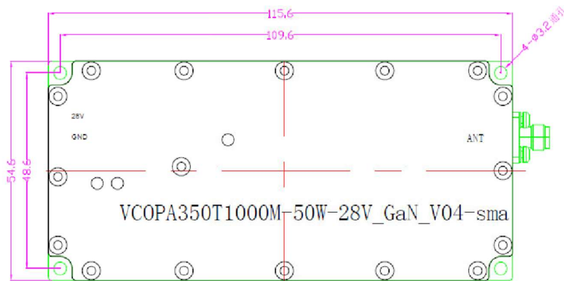
350-1000MHz Drawing
