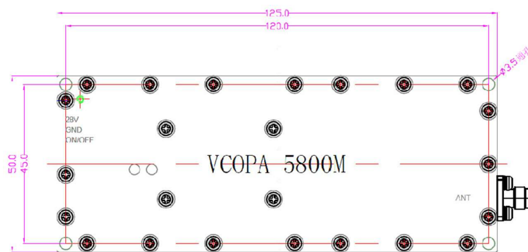
3000-5900MHz Drawing
