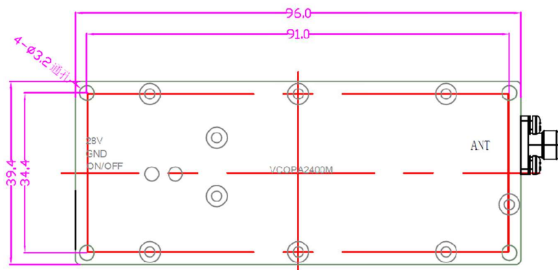
1100-2700MHz Drawing
