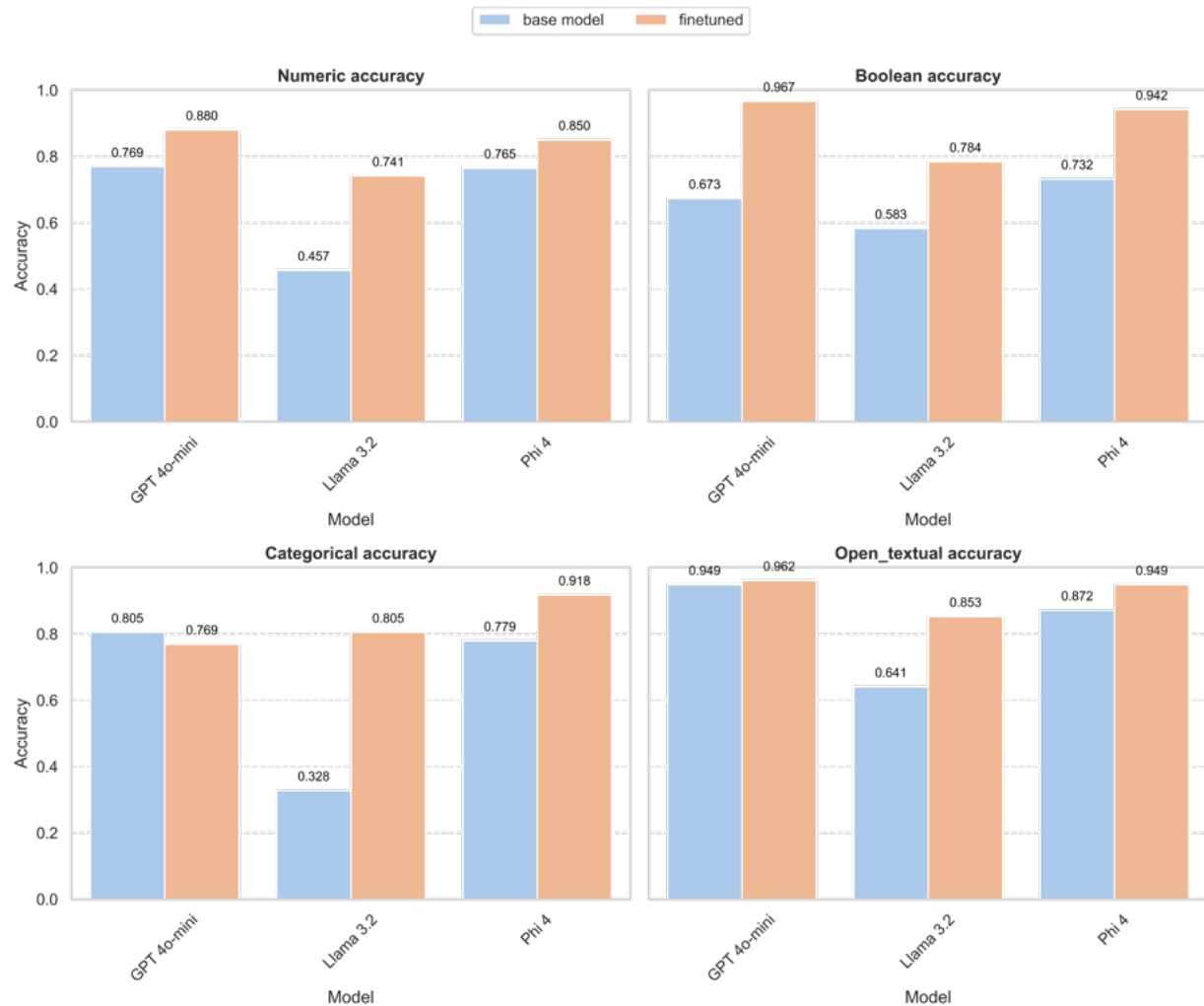
Figure 6: Accuracy comparison - Finetuned models - Kind of datatype
