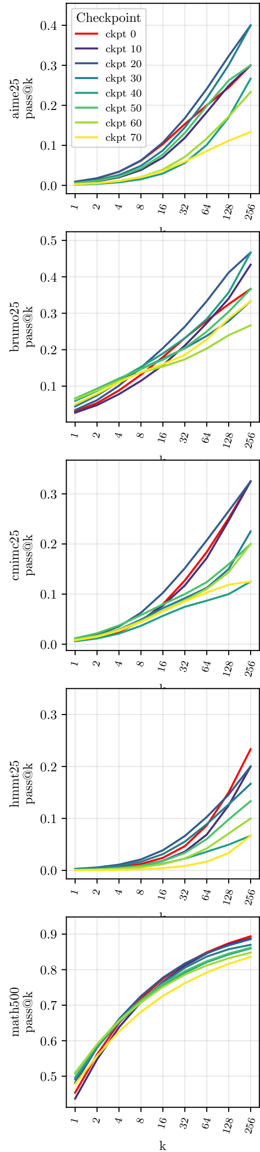
Llama3.1-8B-Instruct, GRPO
