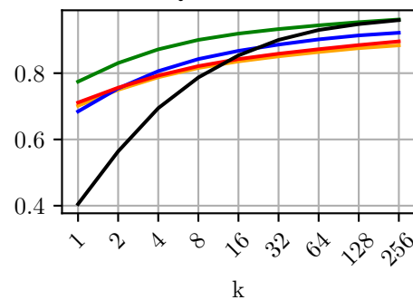
Qwen2.5-7B
