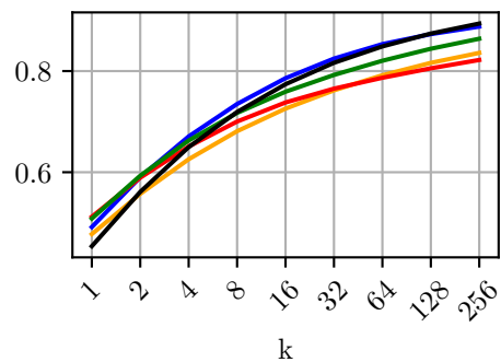
Llama3.1-8B-Instruct
