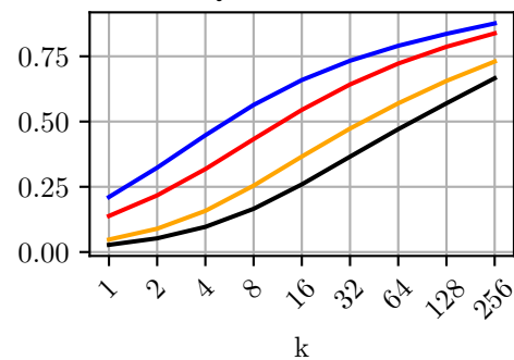
Qwen2.5-1.5B
