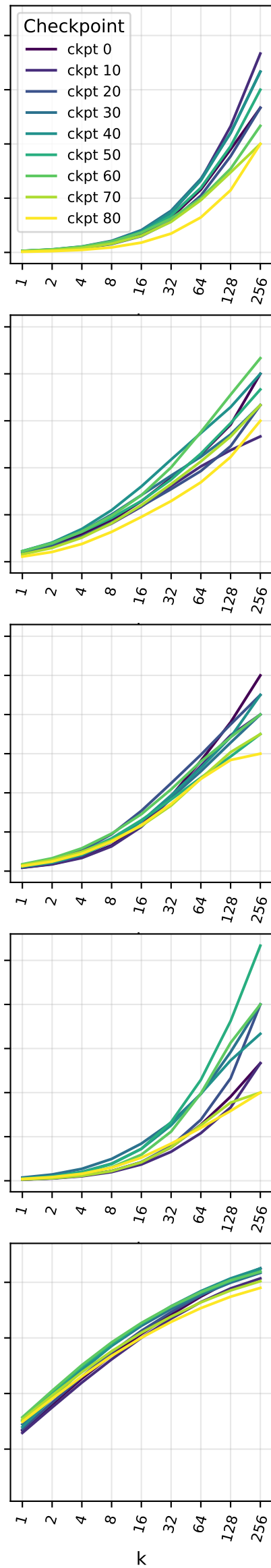
EuroLLM-9B-Instruct, GRPO-S
