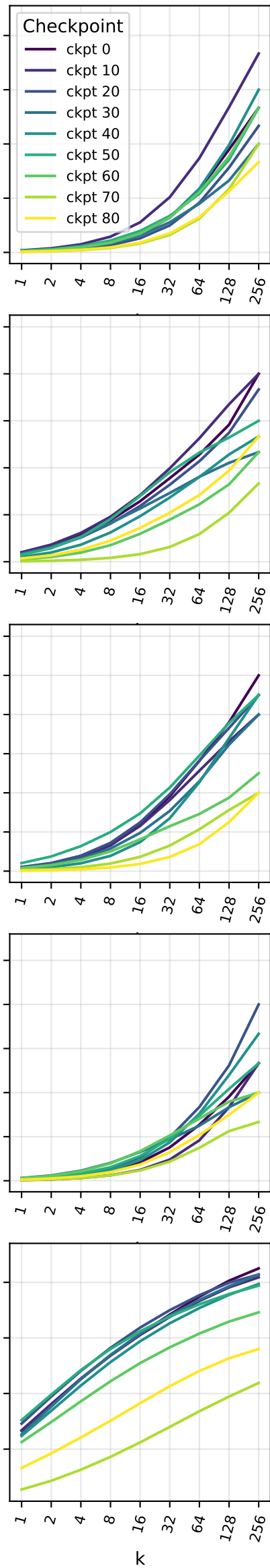
EuroLLM-9B-Instruct, GSPO
