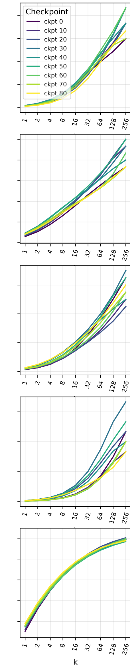
Llama3.1-8B-Instruct, Pass@k Training
