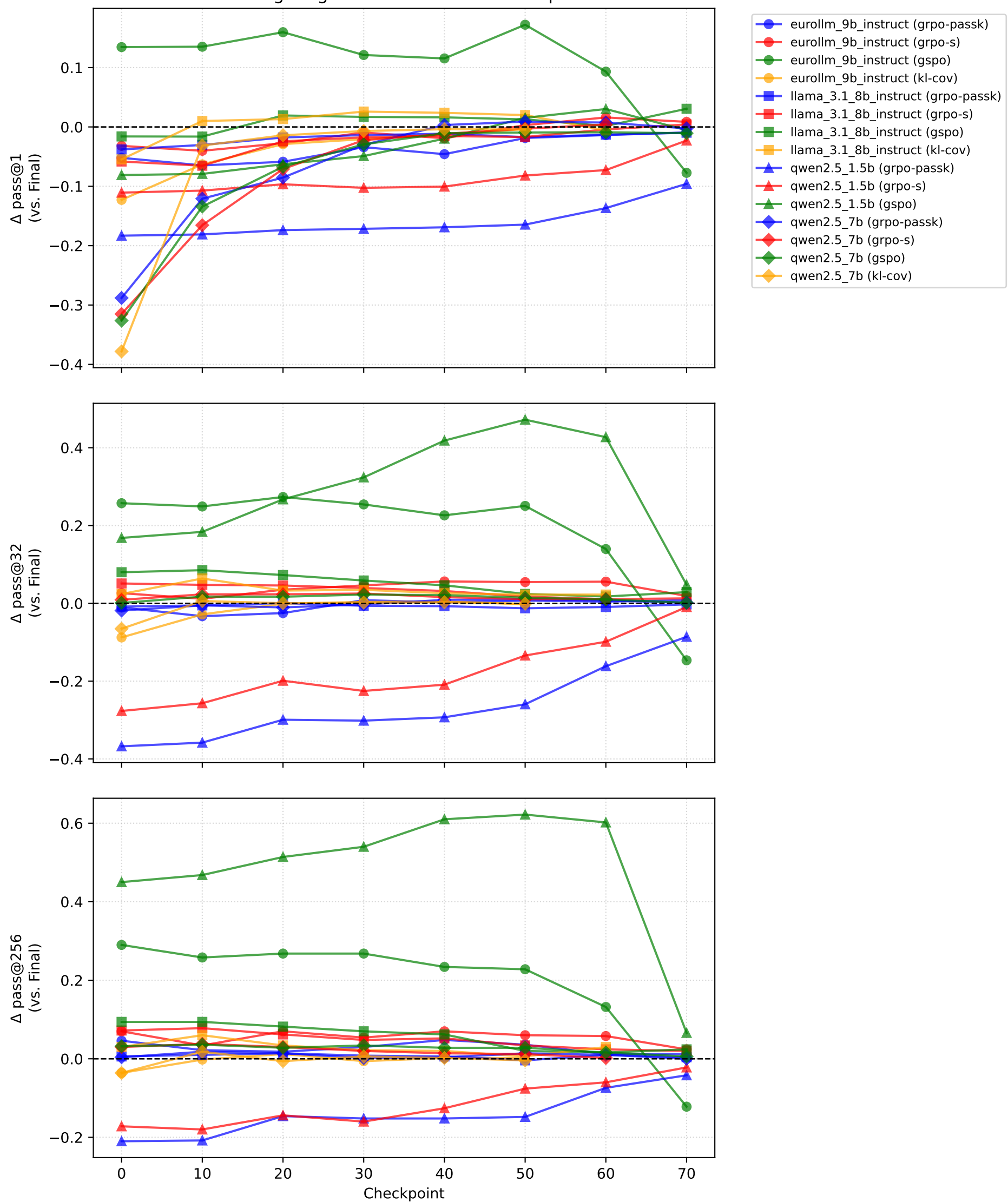
Training Progress: Delta to Final Checkpoint
