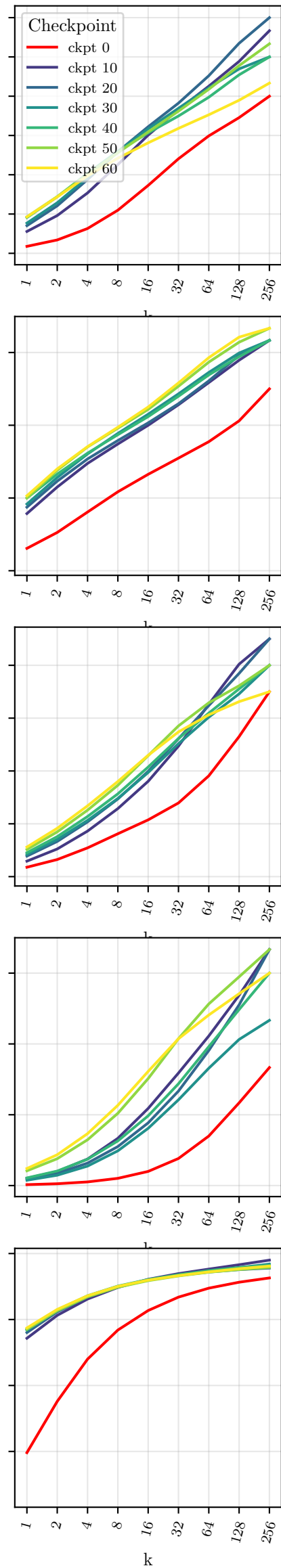
Qwen2.5-7B, KL-Cov
