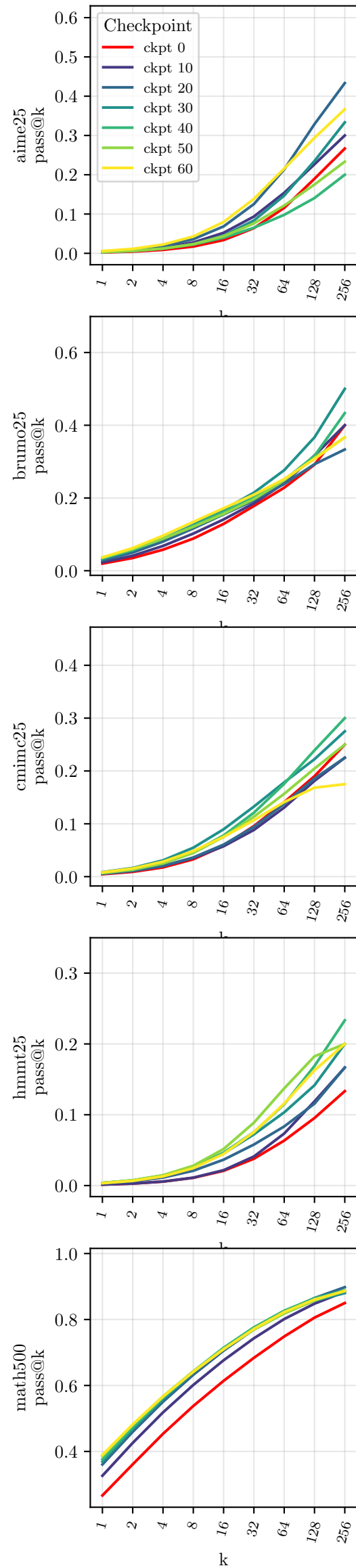
EuroLLM-9B-Instruct, KL-Cov
