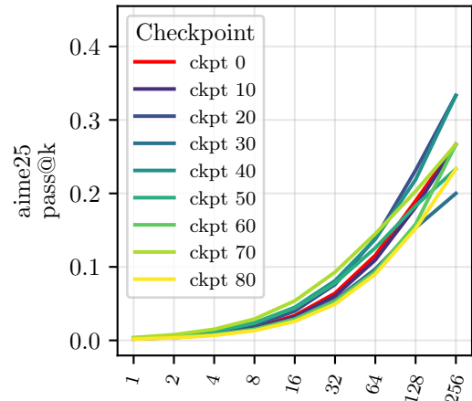
EuroLLM-9B-Instruct, Pass@k Training
