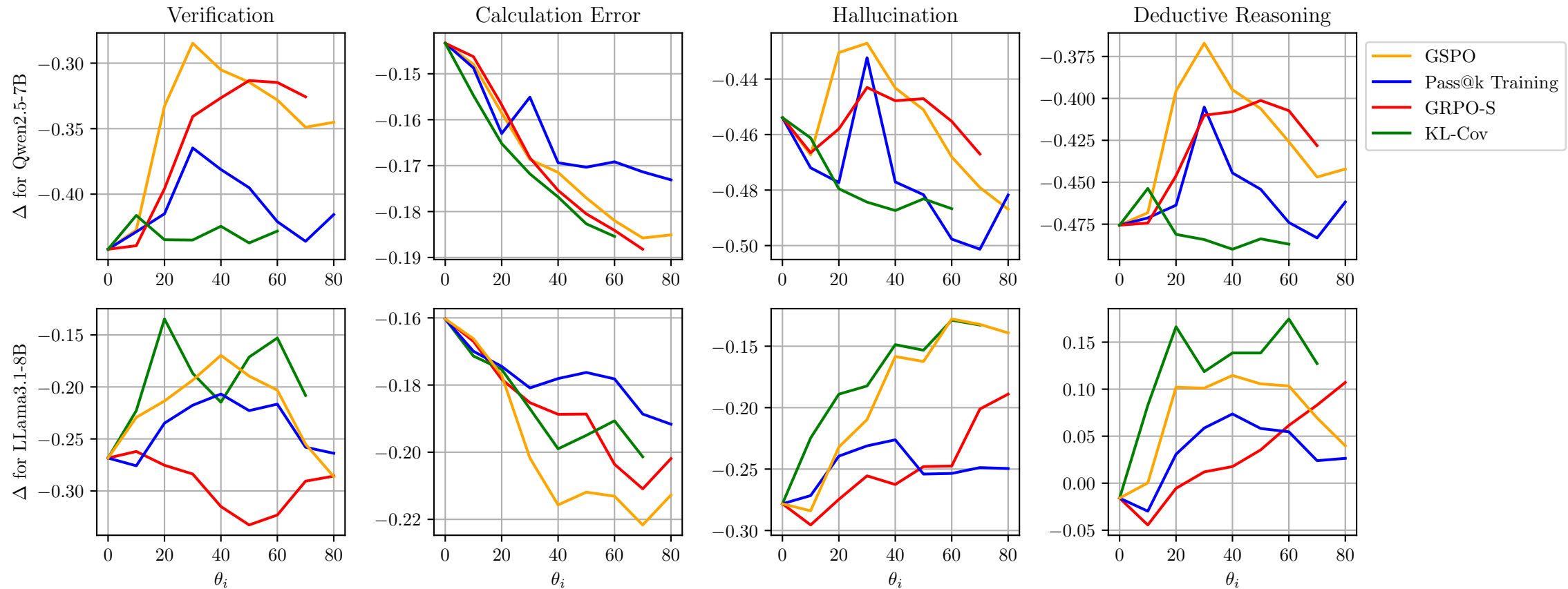
\Delta between Augmentation p(\tilde{x}|\theta_i) and Anchor p(x|\theta_i) for x \approx \tilde{x}
