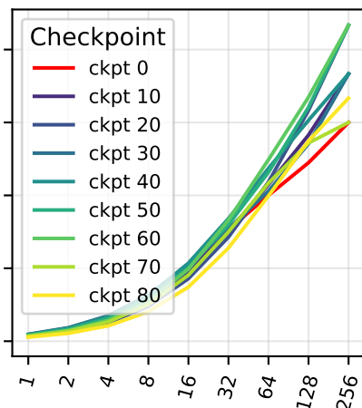
Llama3.1-8B-Instruct, Pass@k Training
