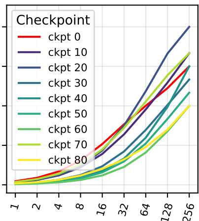
Llama3.1-8B-Instruct, GSPO
