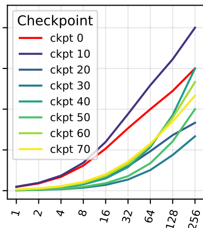
Llama3.1-8B-Instruct, KL-Cov
