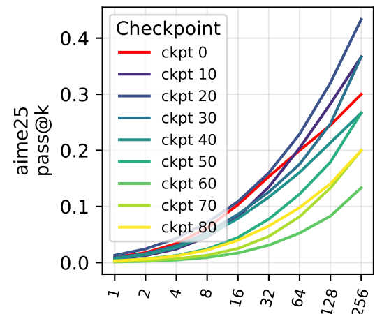
Llama3.1-8B-Instruct, GRPO-S
