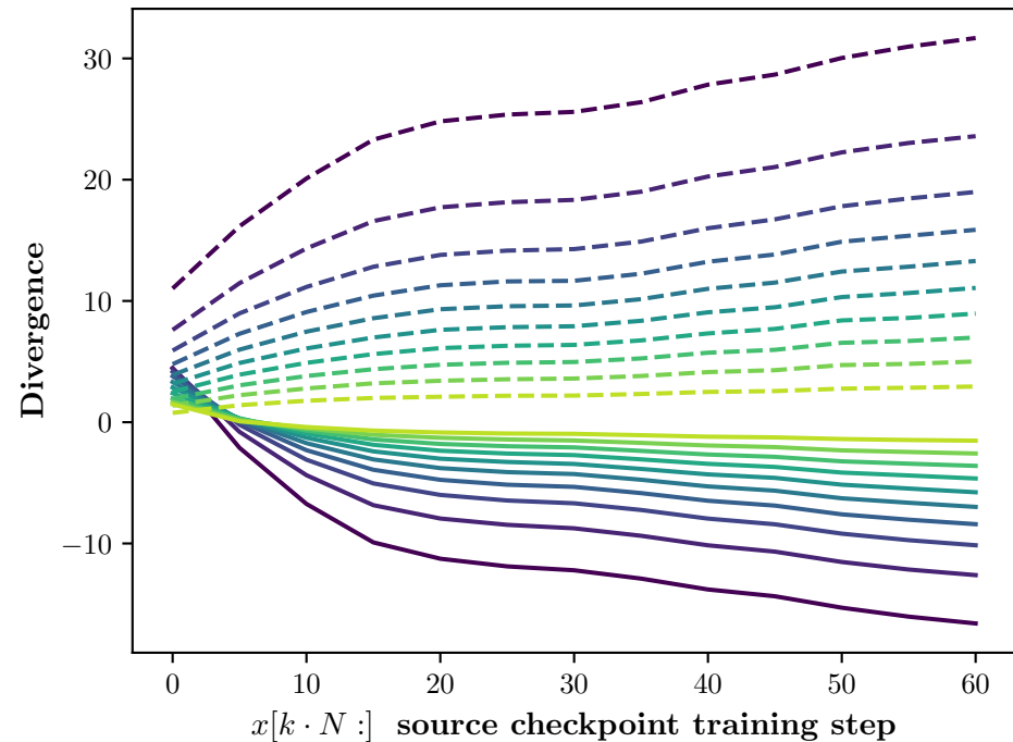
KL-Divergences, Normalized by Sequence Length; Suffix KL-Divergences
