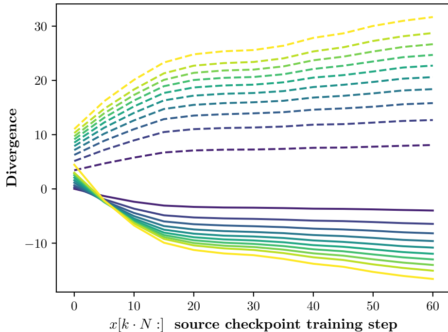
Model: qwen2.5_7b Method: kl-cov Prefix KL-Divergences
