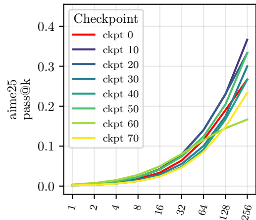
EuroLLM-9B-Instruct, GRPO
