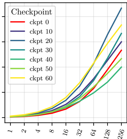
EuroLLM-9B-Instruct, KL-Cov
