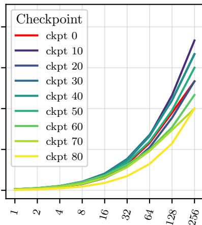
EuroLLM-9B-Instruct, GRPO-S
