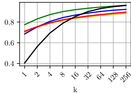
Qwen2.5-7B
