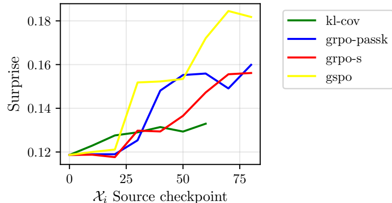
EuroLLM-9B
