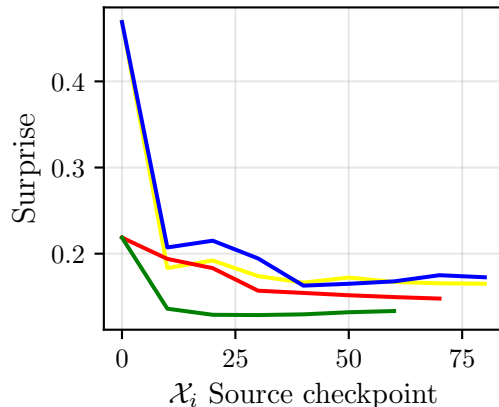
Qwen2.5-7B
