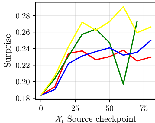
Llama3.1-8B-Instruct
