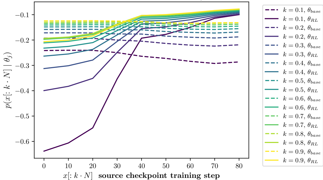
Model: eurollm_9b_instruct Method: grpo-passk Prefix likelihoods p(x[: k \cdot N] | \theta_j)
