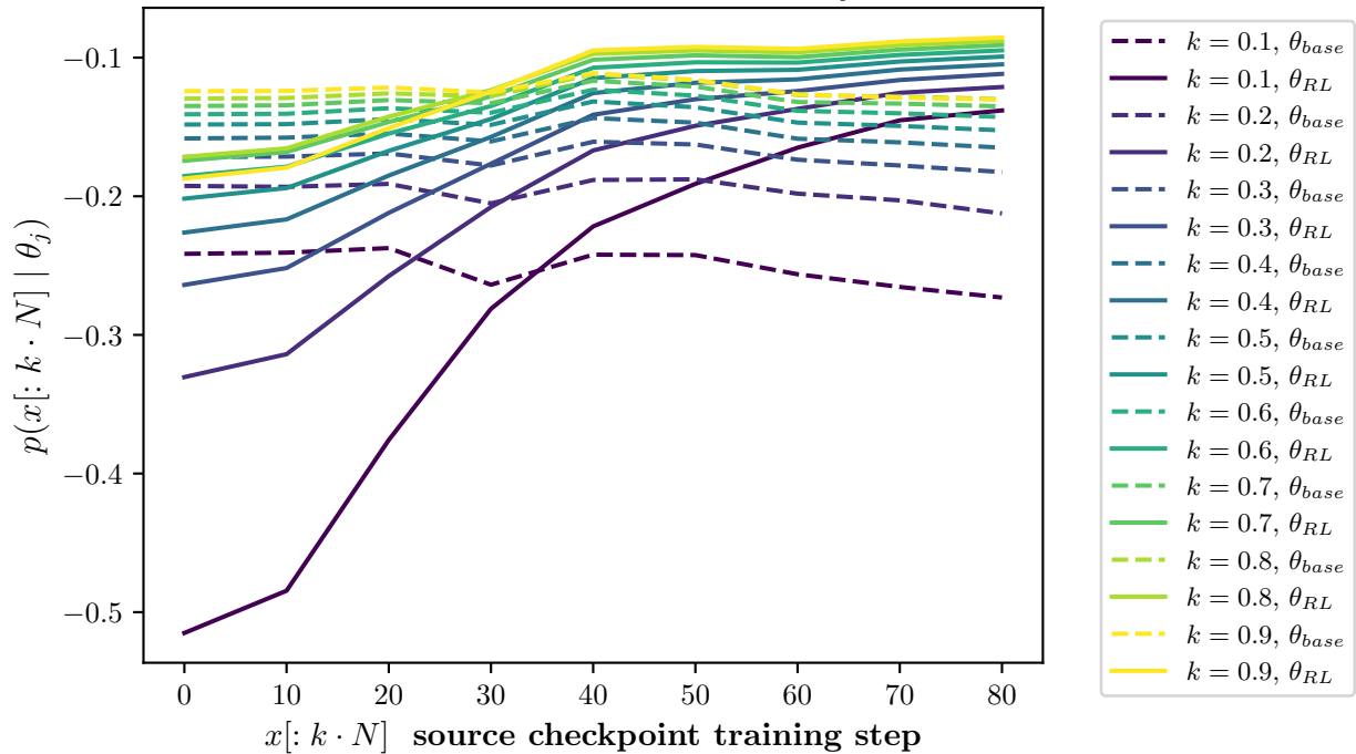
Model: eurollm_9b_instruct Method: grpo-s Prefix likelihoods p(x[: k \cdot N] | \theta_j)
