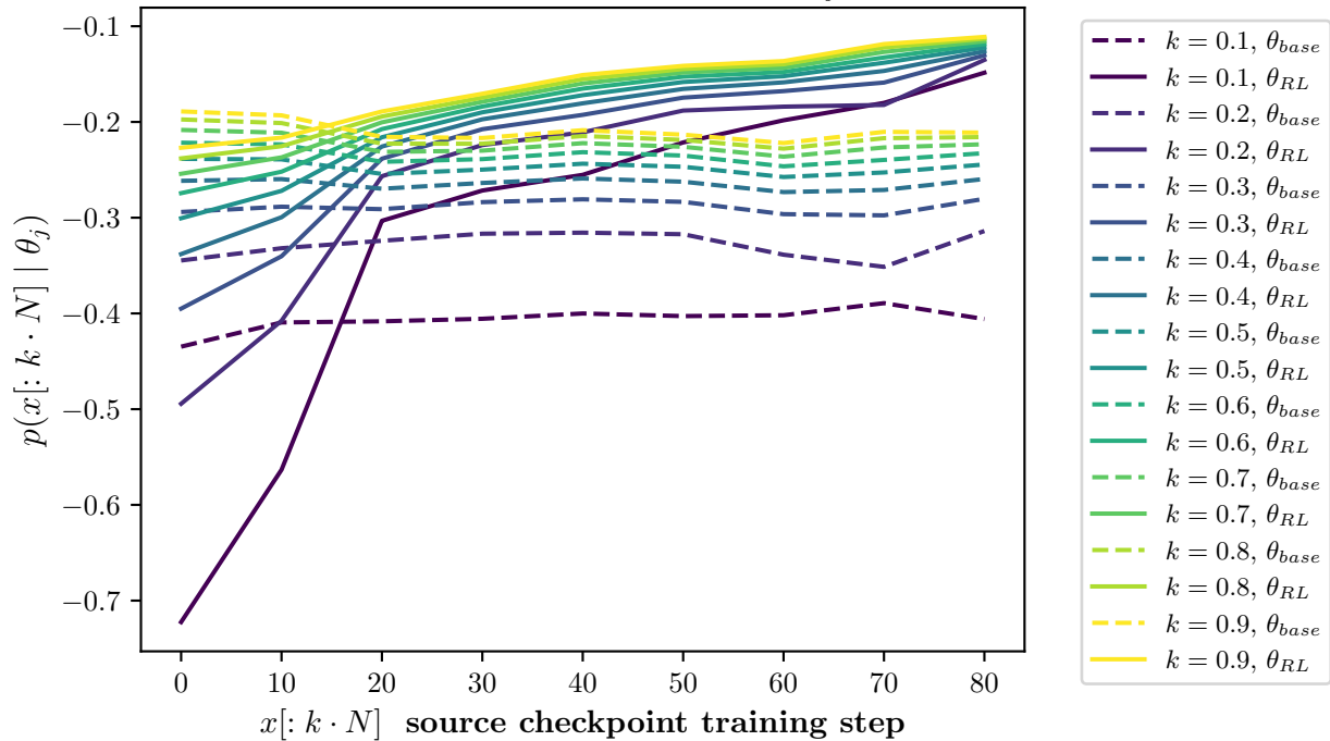
Model: llama_3.1_8b_instruct Method: grpo-s Prefix likelihoods p(x[: k \cdot N] | \theta_j)
