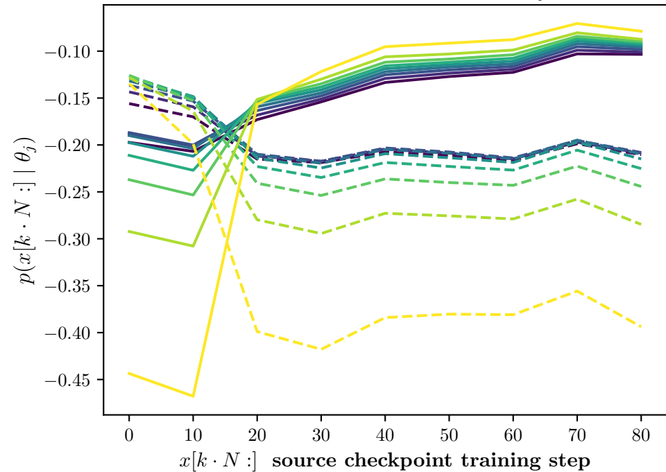
Log-likelihoods of subsequences, Normalized by Sequence Length; Suffix likelihoods p(x[k \cdot N :] | \theta_j)
