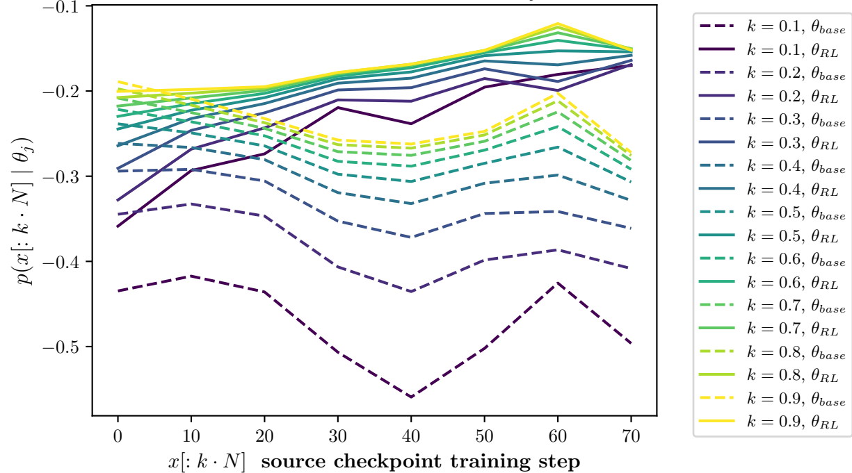
Model: llama_3.1_8b_instruct Method: kl-cov Prefix likelihoods p(x[: k \cdot N] | \theta_j)
