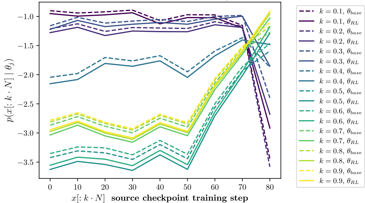
Model: qwen2.5_1.5b Method: grpo-passk Prefix likelihoods p(x[: k \cdot N] | \theta_j)
