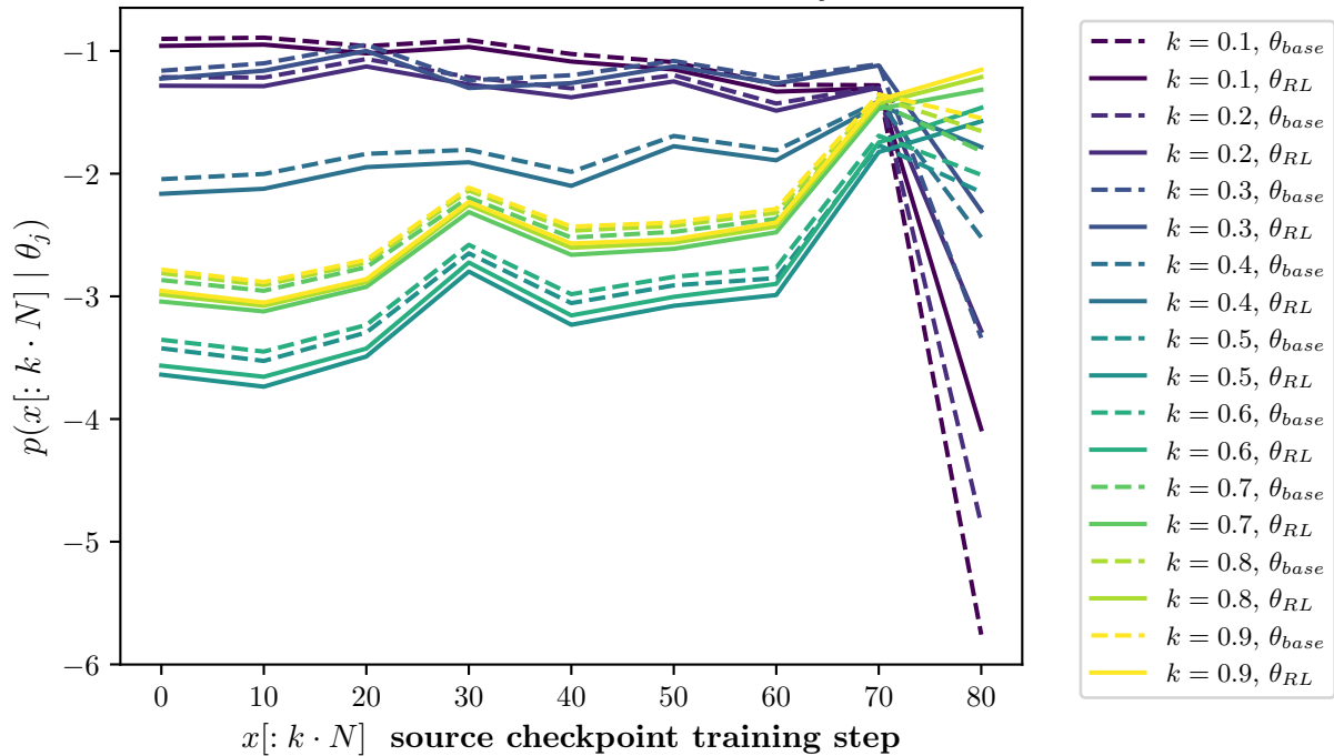
Model: qwen2.5_1.5b Method: grpo-s Prefix likelihoods p(x[: k \cdot N] | \theta_j)
