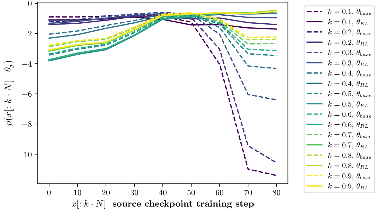
Model: qwen2.5_1.5b Method: gspo Prefix likelihoods p(x[: k \cdot N] | \theta_j)
