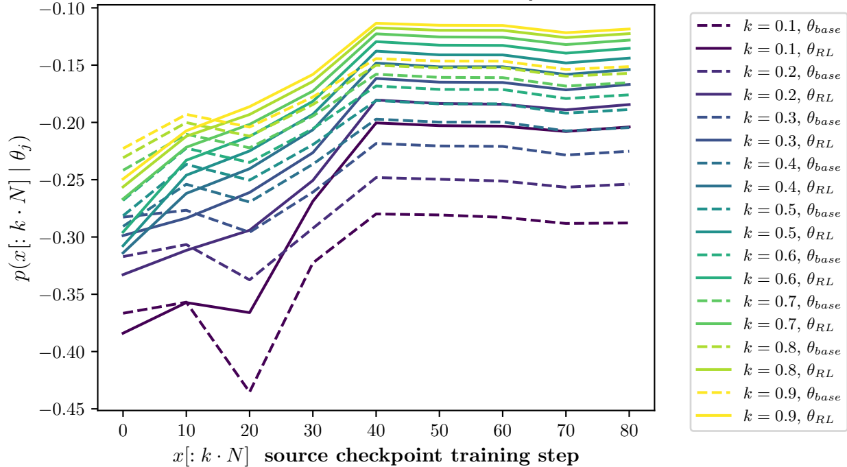
Model: qwen2.5_7b Method: grpo-passk Prefix likelihoods p(x[: k \cdot N] | \theta_j)
