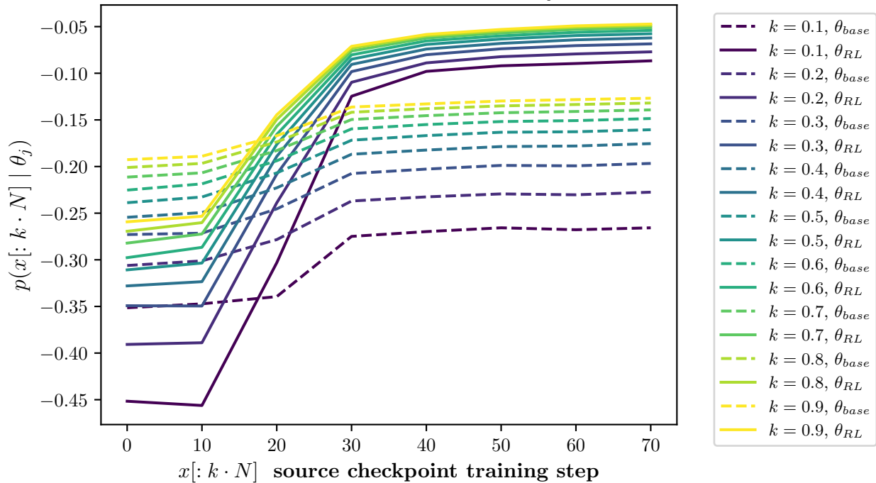
Model: qwen2.5_7b Method: grpo-s Prefix likelihoods p(x[: k \cdot N] | \theta_j)
