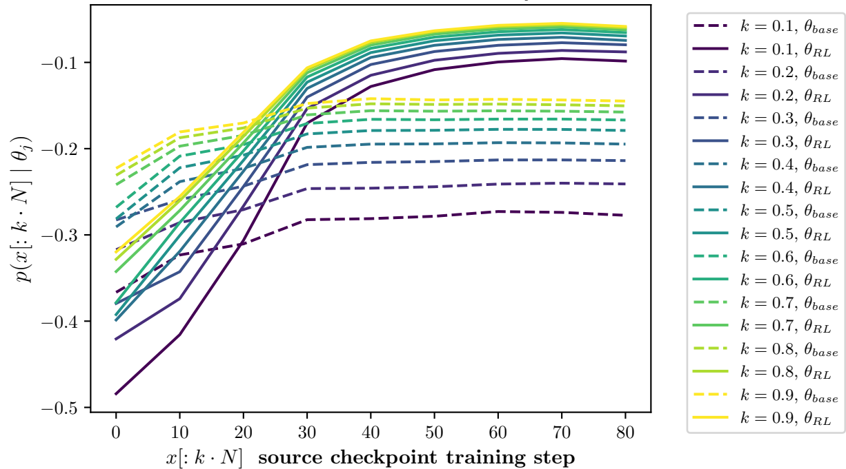
Model: qwen2.5_7b Method: gspo Prefix likelihoods p(x[: k \cdot N] | \theta_j)
