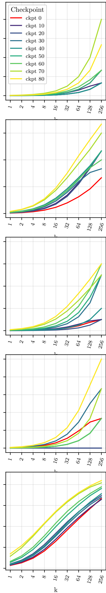
Qwen2.5-1.5B, GRPO-S
