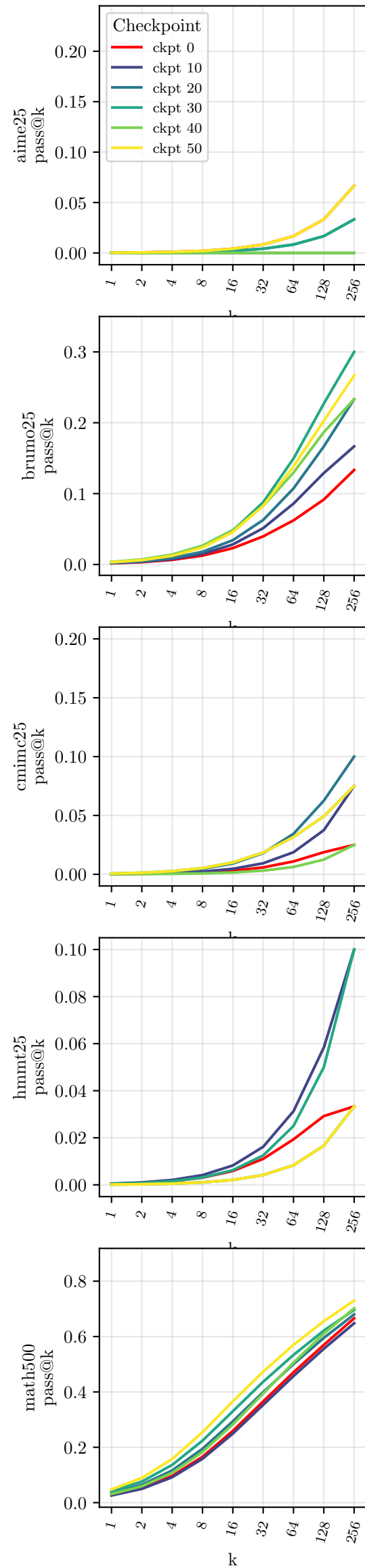
Qwen2.5-1.5B, GRPO
