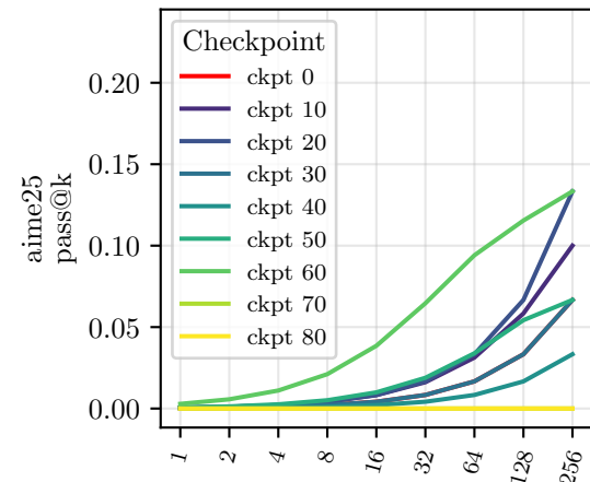
Qwen2.5-1.5B, GSPO
