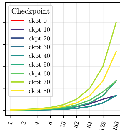
Qwen2.5-1.5B, GRPO-S
