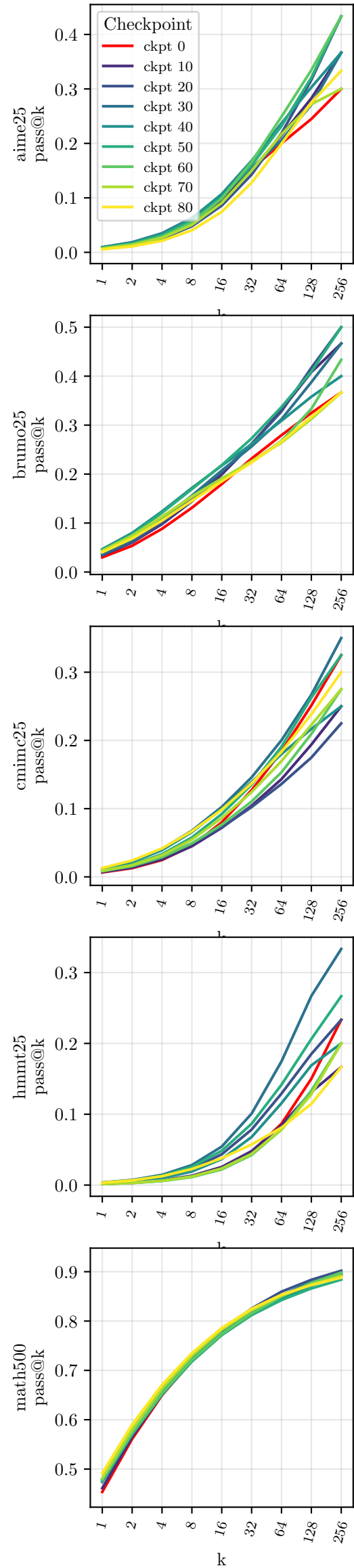
Llama3.1-8B-Instruct, Pass@k Training
