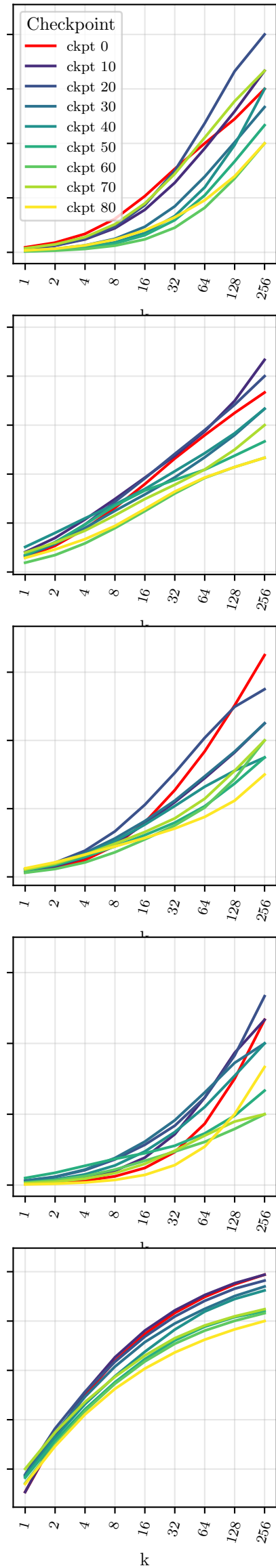
Llama3.1-8B-Instruct, GSPO
