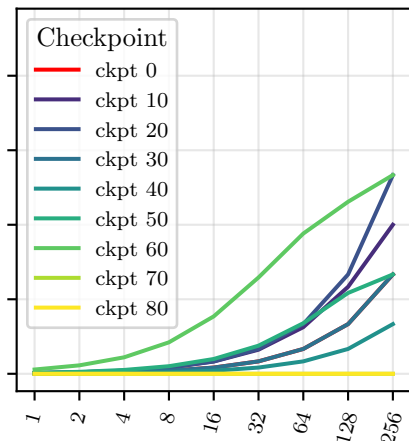
Qwen2.5-1.5B, GSPO
