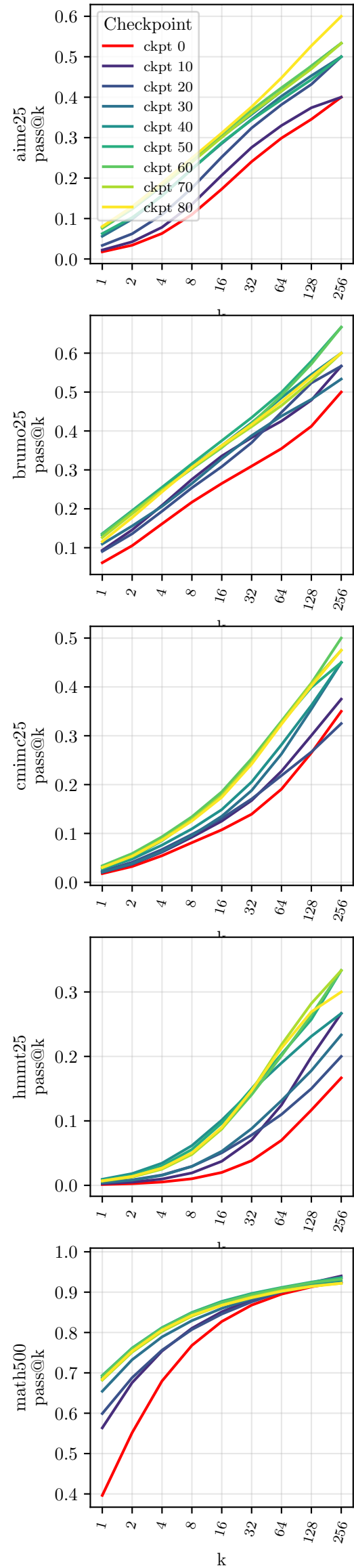
Qwen2.5-7B, Pass@k Training
