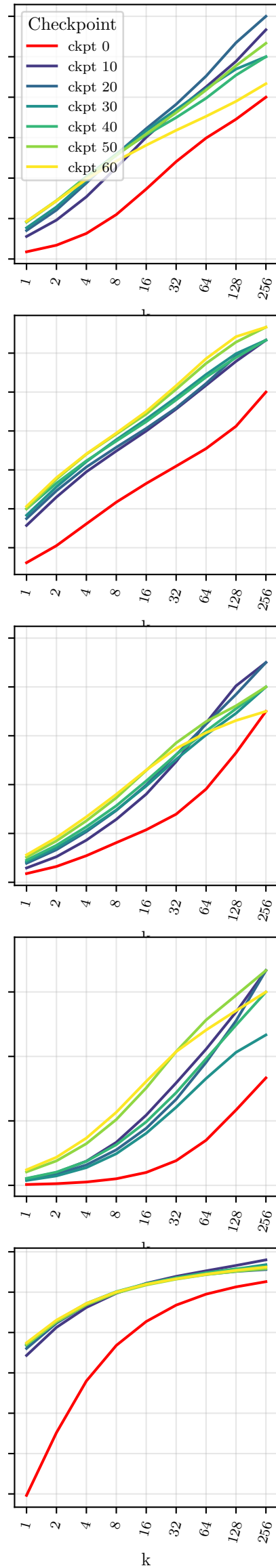
Qwen2.5-7B, KL-Cov
