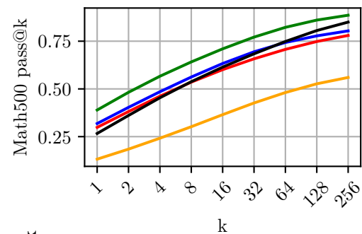
EuroLLM-9B-Instruct
