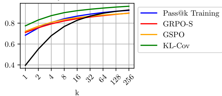
Qwen2.5-7B
