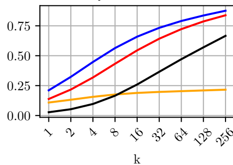
Qwen2.5-1.5B
