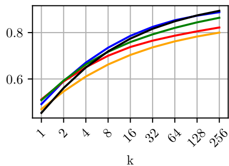
Llama3.1-8B-Instruct
