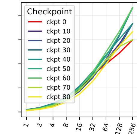
Llama3.1-8B-Instruct, Pass@k Training
