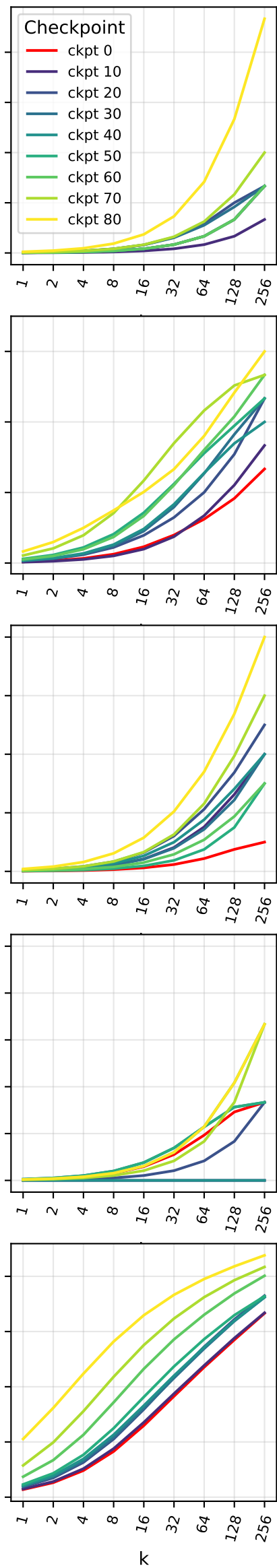
Qwen2.5-1.5B, Pass@k Training
