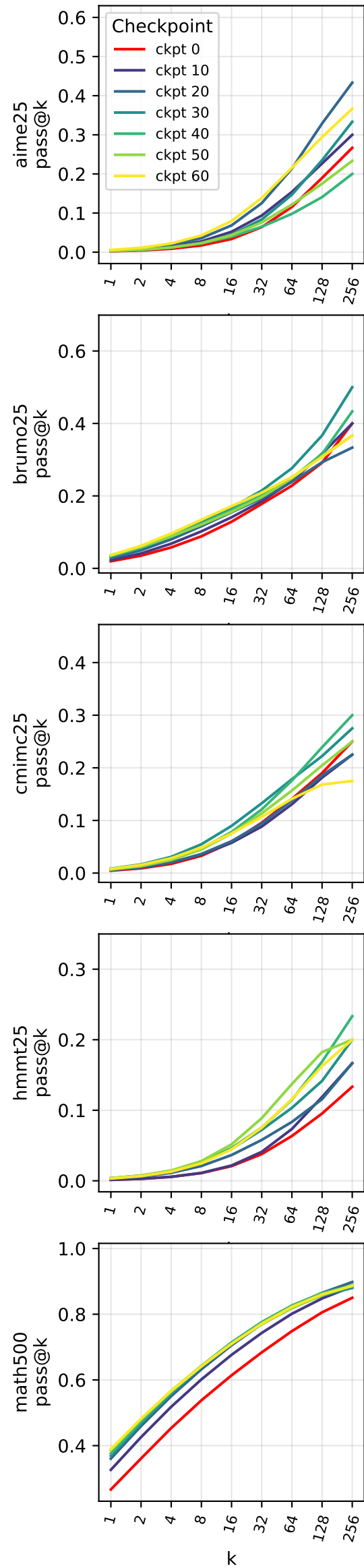
EuroLLM-9B-Instruct, KL-Cov
