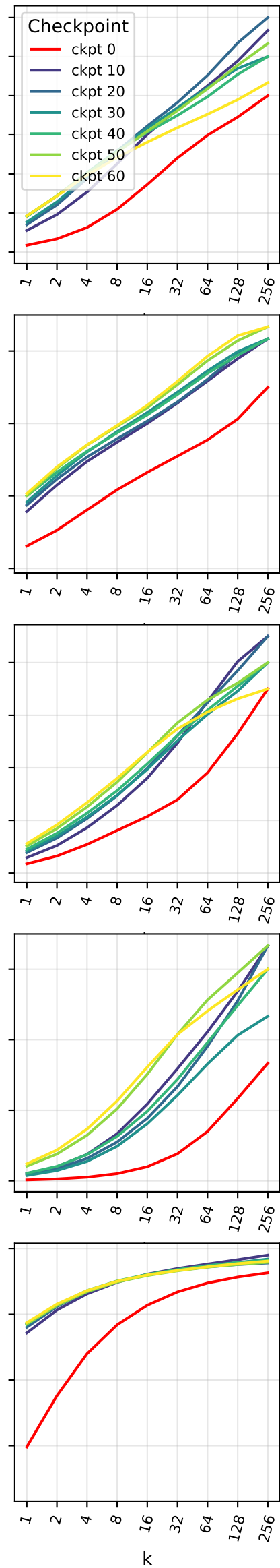
Qwen2.5-7B, KL-Cov
