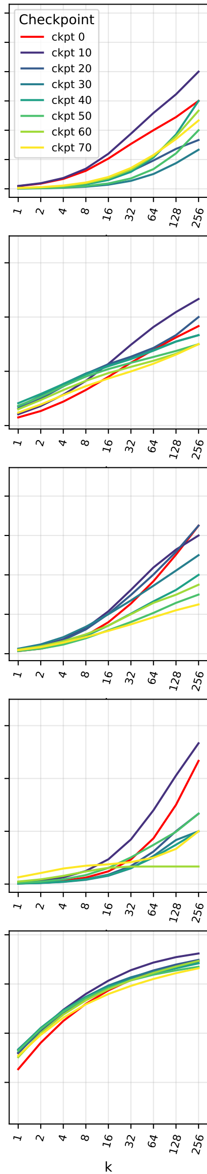
Llama3.1-8B-Instruct, KL-Cov
