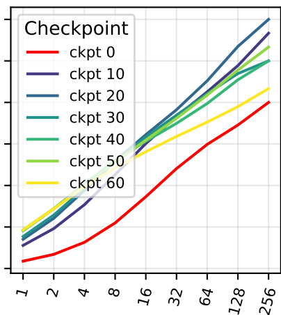
Qwen2.5-7B, KL-Cov
