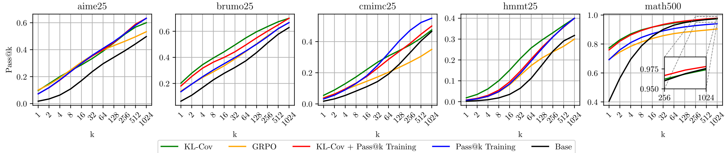
Pass@k for different Datasets
