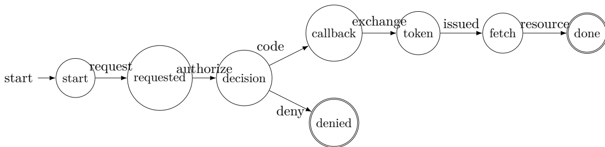
Figure 5.2: OAuth state machine derived from legal grammar continuations.
