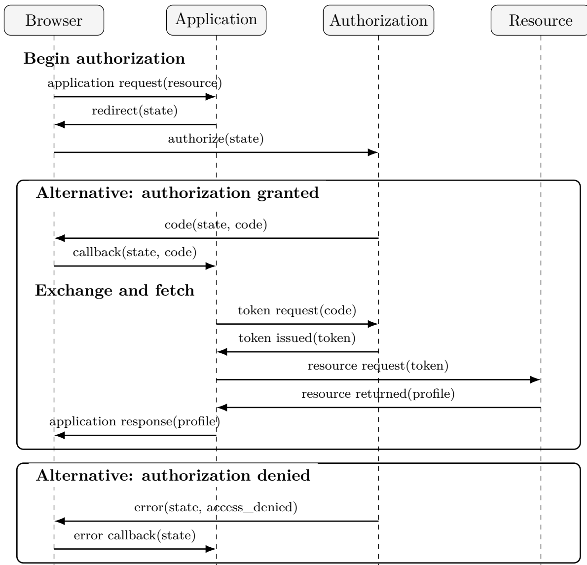
Figure 5.1: OAuth interaction view. The frames bracket the two alternatives after the common authorization prefix; only the granted branch continues to token exchange and resource access.
