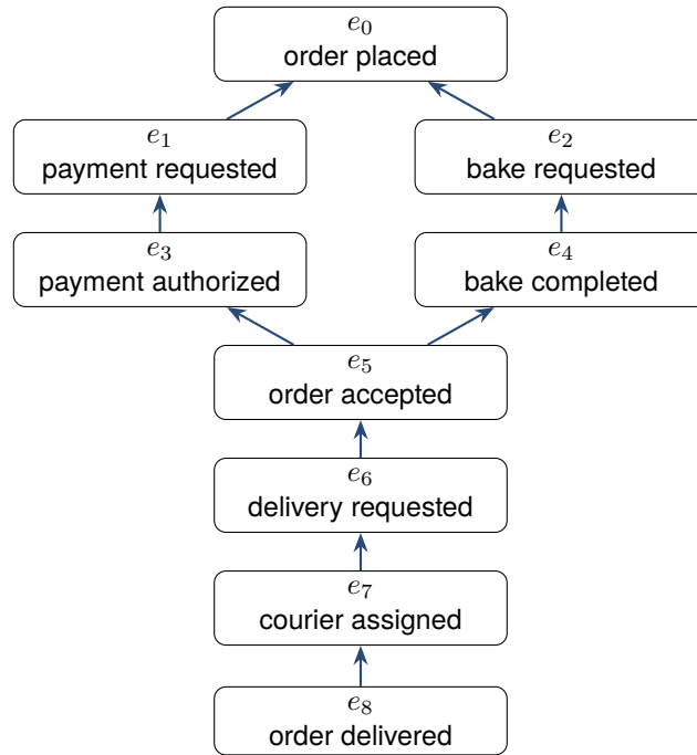
Figure 2.1: The table’s immediate causal backpointers rendered as a graph. Each arrow points from an event to an ID in its priorIds list: for example, e_2 \rightarrow e_0 . The two arrows from e_5 expose the payment/baking join.
