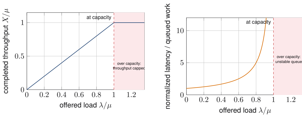
Figure 5.3: Offered-load capacity. Beyond \lambda/\mu = 1 , throughput cannot increase but queued work and latency continue to worsen until backpressure, rejection, an outage, or fatal memory exhaustion intervenes.
