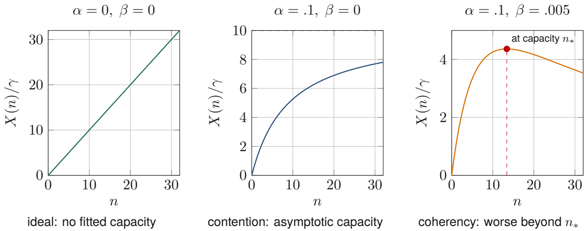
Figure 5.2: Universal Scalability Law regimes. \gamma rescales every vertical axis. Contention alone saturates; coherency creates a finite peak and declining throughput beyond capacity.
