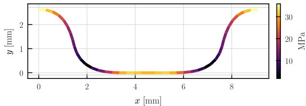
S8 (C039), deformed stress field
