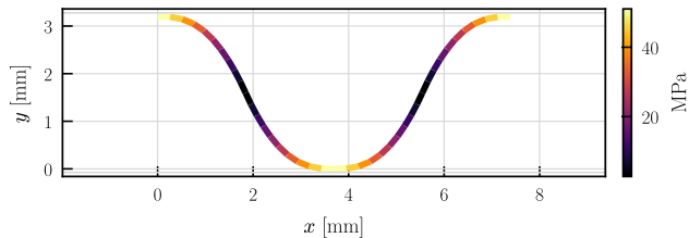
S5 (C038), deformed stress field
