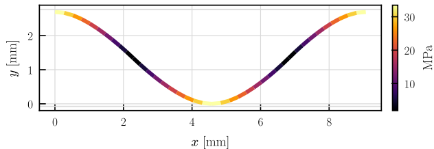
S8 (C039), deformed stress field
